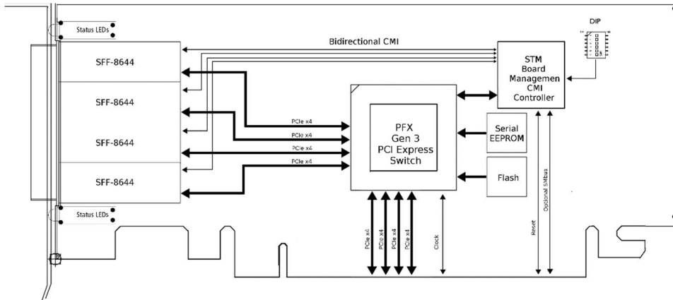
Figure 5: PCI-AD-X16HE-PS-MD Simplified Schematics
