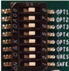
Figure 1: DIP Switch
